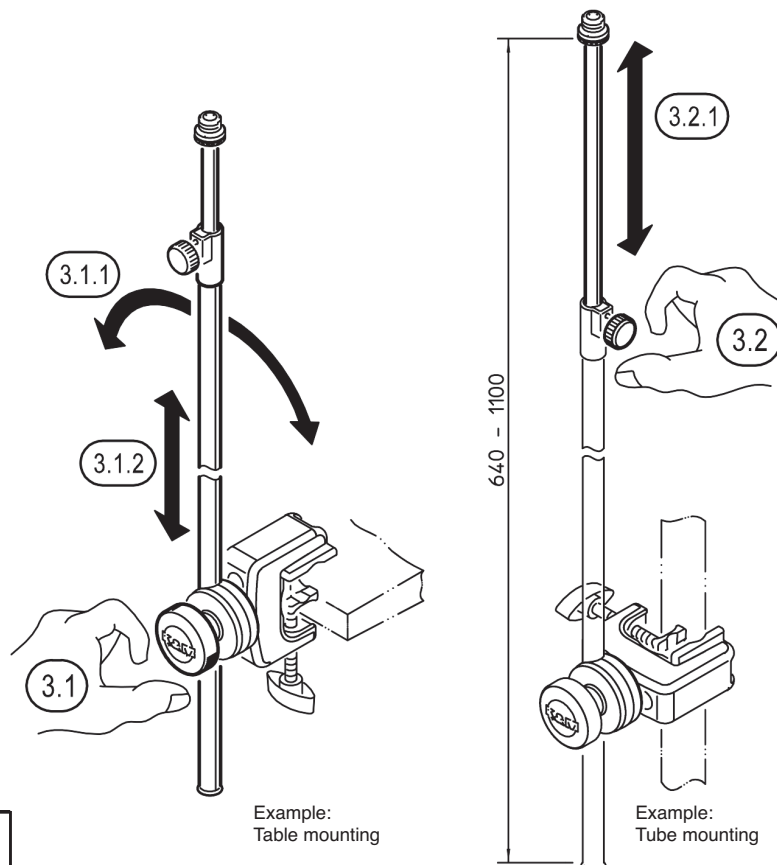
1. COMPONENTS and ASSEMBLY
